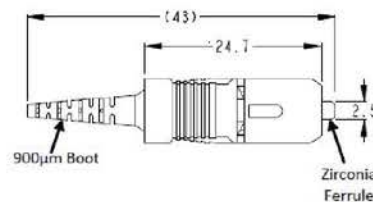
SC Simplex Connector with 900µm Boot
